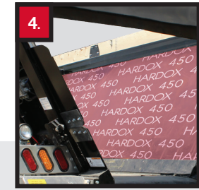
4. Our hopper bodies inside sheathing comes standard with 1/8" 450 Hardox material. Our seal plates are also made of the same material.
